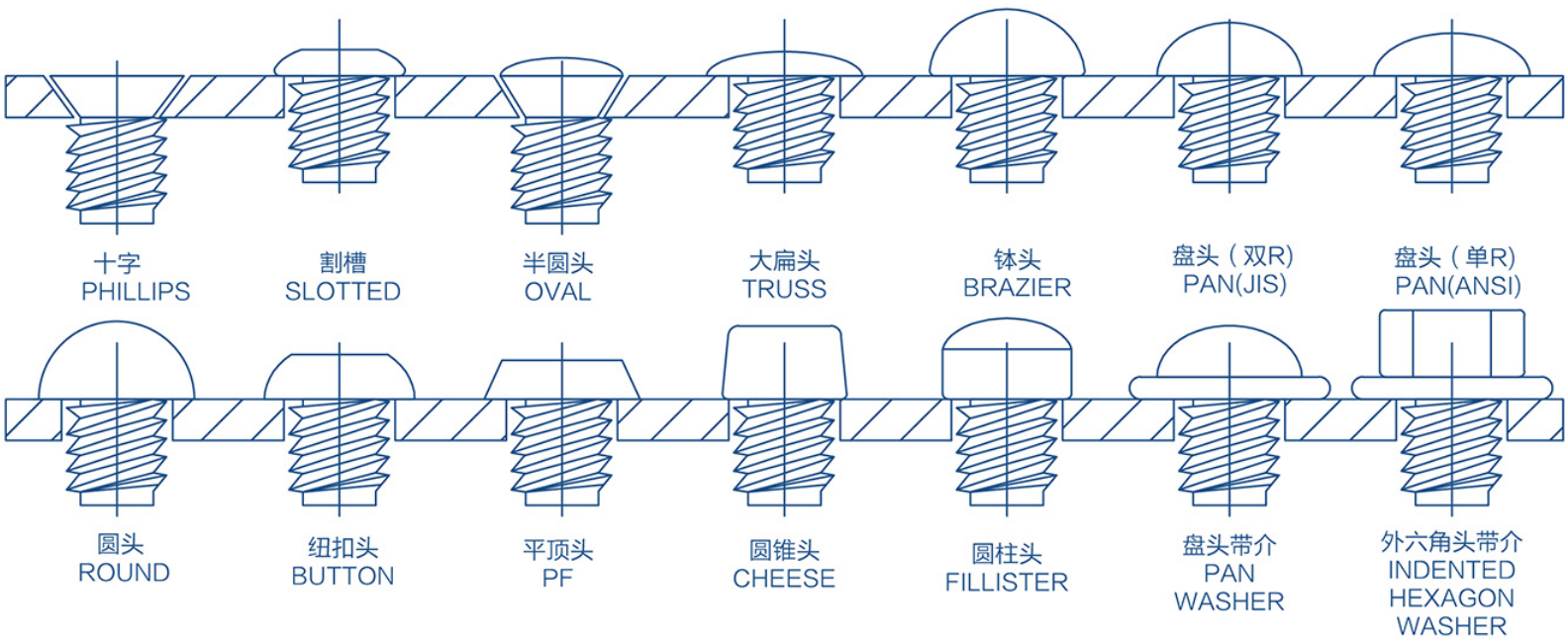
SCREW DRIVERS (槽型对照表)
